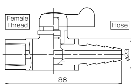
● Female Thread×Hose
