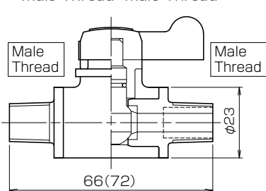
● Male Thread×Male Thread
