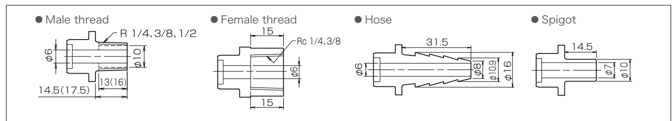
● Male Thread×Hose
