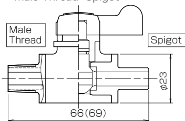
● Male Thread×Spigot
