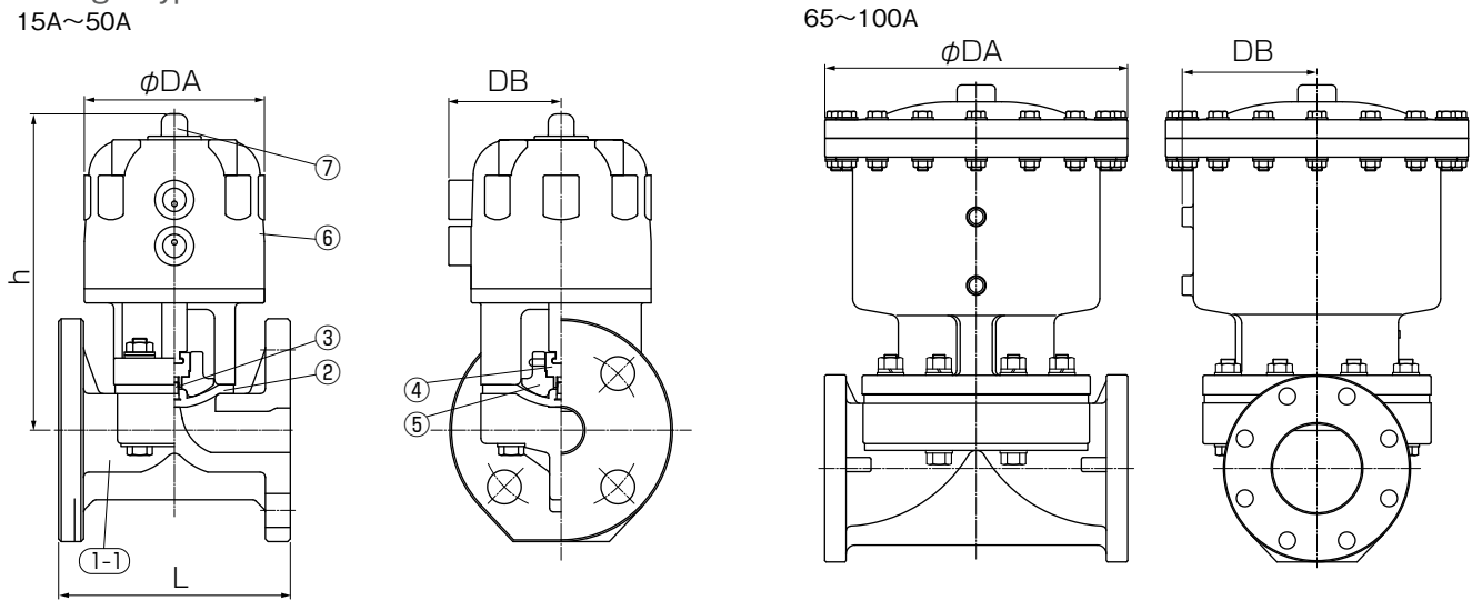
Figure (Flange Type · TS Socket Type · Thread Type · Butt Type)
