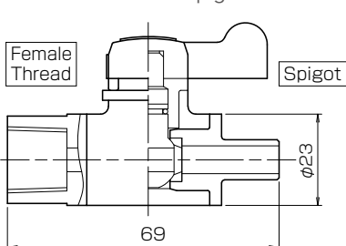
● Female Thread×Spigot
