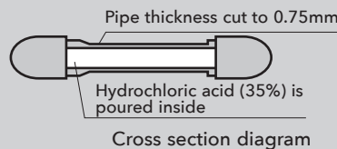
Cross section diagram
